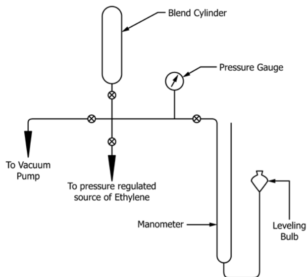
FIG. 2 Gas-Blending Manifold
